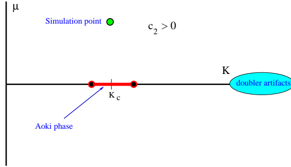
Fig. 11.6. Continuing around the Aoki phase with twisted mass. This sketch considers the case c_2 > 0 where the parity broken phase extends over a region along the kappa axis. Figure taken from Ref. [109].
