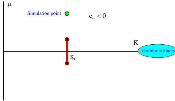
Fig. 11.7. As in Fig. 11.6, but for the case c_2 < 0 so the chiral transition on the kappa axis becomes first order. Figure taken from Ref. [109].
