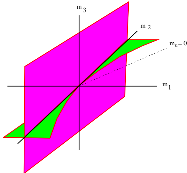
Fig. 10.9. The full phase diagram for two-flavor QCD as a function of the three mass parameters. It consists of two intersecting first order surfaces with a second order edge along curves satisfying m_3 = 0 , |m_1| < |m_2| . There is no structure along the m_u = 0 line except when both quark masses vanish. Figure from Ref. [99]
