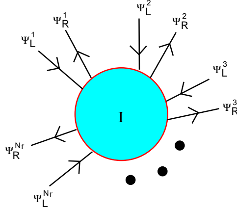
Fig. 9.5. The 't Hooft vertex for N_f flavors is a 2N_f effective fermion operator that flips the spin of every flavor.
