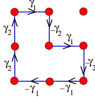
Fig. 12.2. When a fermion circumnavigates a loop in the naive formulation, it picks up a factor that always involves an even power of any particular gamma matrix. Figure from Ref. [127].
