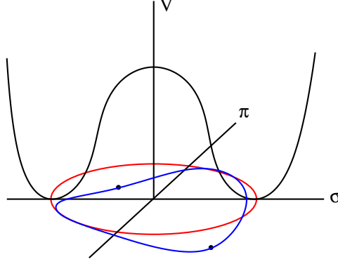
Fig. 10.6. The m_2 and m_3 terms warp the Mexican hat potential into two separate minima. The direction of the warping is determined by the relative size of these parameters. Figure taken from Ref. [99].
