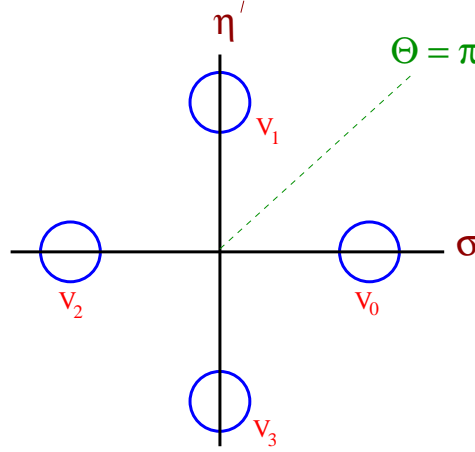
Fig. 10.1. With massive quarks and a twisting angle of \phi = \pi/N_f , two of the minima in the \sigma, \eta' plane become degenerate. This corresponds to a first order transition at \Theta = \pi .
