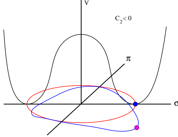
Fig. 11.3. Lattice artifacts could quadratically warp the effective potential. If this warping is downward in the sigma direction, the chiral transition becomes first order without the pions becoming massless. Figure taken from Ref. [109].
