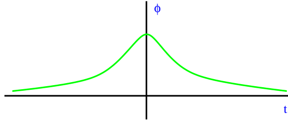
Fig. 7.2. The adiabatic evolution gives rise to a normalizable zero mode of the four dimensional Dirac operator.
