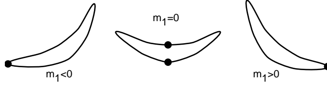
Fig. 10.7. In the m_1, m_2 plane, m_{\pi_0}^2 can pass through zero, giving rise to pion condensation at an Ising-like transition. Figure taken from [30].
