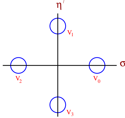
Fig. 9.2. For four massless flavors we have four equivalent minima in the \sigma, \eta' plane. This generalizes to N_f minima with N_f flavors.
