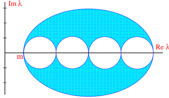
Fig. 11.1. The eigenvalue spectrum of the free Wilson fermion operator is a set of nested circles. On turning on the gauge fields, some eigenvalues drift into the open regions. Some complex pairs can collide and become real. These are connected to gauge field topology. Figure taken from Ref. [109].
