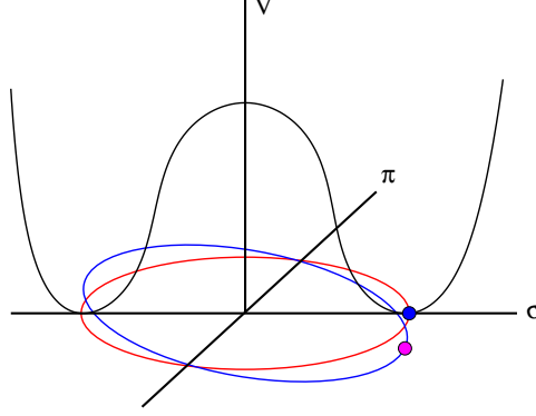
Fig. 8.3. A small quark mass term tilts the effective potential, selecting one direction for the true vacuum and giving the Goldstone bosons a mass proportional to the square root of the quark mass.
