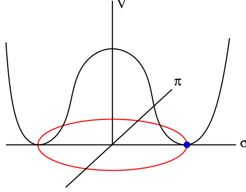
Fig. 8.2. The flavor non-singlet pseudoscalar mesons are Goldstone bosons corresponding to flat directions in the effective potential.
