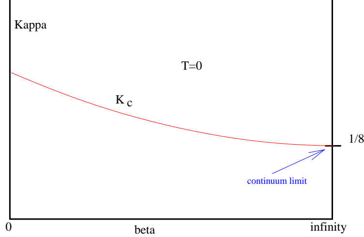
Fig. 11.2. The continuum limit of lattice gauge theory with Wilson fermions occurs at \beta \rightarrow \infty and K \rightarrow 1/8 . Coming in from this point to finite beta is the curve K_c(\beta) , representing the lowest phase transition in K for fixed beta. The nature of this phase transition is a delicate matter, discussed in the text. Figure taken from Ref. [109].
