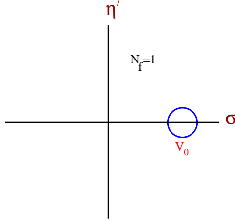
Fig. 10.3. The effective potential for one-flavor QCD with small quark mass has a unique minimum in the \sigma, \eta' plane. The minimum is shifted from zero due to the effect of the 't Hooft vertex.
