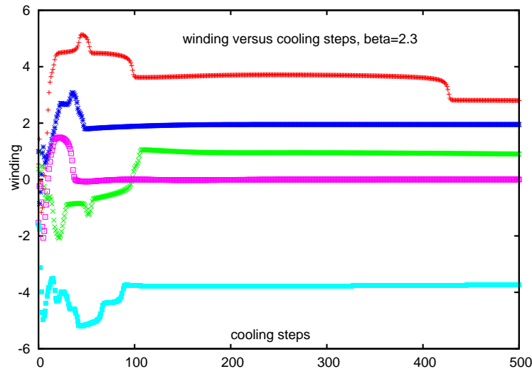
Fig. 13.1. The winding number as a function of cooling steps for a set of 5 lattices of size 16^4 at \beta = 2.3 . Note how it settles into approximately integer values with occasional jumps between different windings. Figure from Ref. [164].
