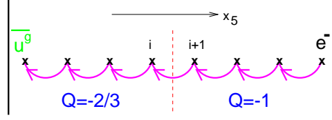
Fig. 13.3. Pairing the electron with the anti-green-up-quark. Figure taken from [180].
