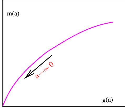
Fig. 6.1. In the continuum limit both the bare coupling and bare mass for QCD flow to zero.
