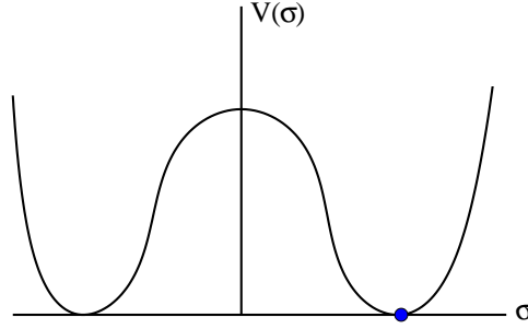
Fig. 8.1. Spontaneous chiral symmetry breaking is represented by a double well effective potential with the vacuum settling into one of two possible minima. In this minimum chiral symmetry is broken by the selection of a specific value for the quark condensate.
