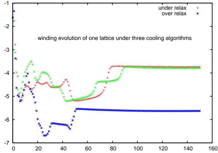
Fig. 13.2. The topological charge evolution for three different cooling algorithms on a single \beta = 2.3 lattice configuration for SU(2) on a 16^4 lattice. Figure from Ref. [164]. With the higher winding numbers, lattice artifacts shift the plateaus slightly away from integer values.
