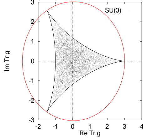
Fig. 9.3. The real and imaginary parts for the traces of 10,000 randomly chosen SU(3) matrices. All points lie within the boundary representing matrices of the form \exp(i\phi\lambda_8) . The tips of the three points represent the center of the group. The outer curve represents the boundary that would be found if the group was the full U(1) . Taken from Ref. [30].
