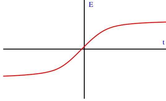
Fig. 7.1. An energy eigenvalue that changes in sign between the distant past and future.
