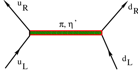
Fig. 10.4. Both pion and eta-prime exchange contribute to spin flip scattering between up and down quarks. Figure from Ref. [99].
