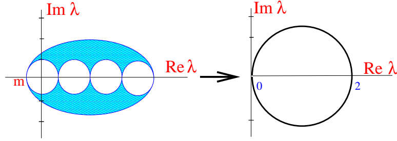
Fig. 12.1. The overlap operator is constructed by projecting the eigenvalues of the Wilson operator onto a circle. Figure taken from Ref. [142].
