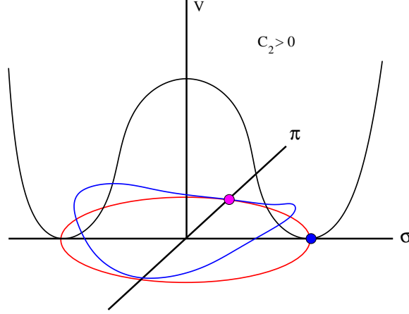
Fig. 11.4. If the lattice artifacts warping the potential upward in the sigma direction, the chiral transition splits into two second order transitions separated by a phase where the pion field has an expectation value. Figure taken from Ref. [109].
