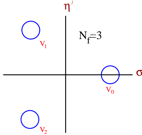
Fig. 10.2. For odd N_f , such as the three flavor case sketched here, QCD is not symmetric under changing the sign of the quark mass. Negative mass corresponds to taking \Theta = \pi .
