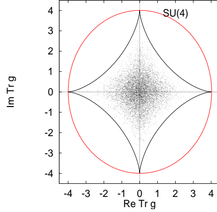
Fig. 9.4. The generalization of Fig. 9.3 to SU(4) . The real and imaginary parts for the traces of 10,000 randomly chosen SU(4) matrices. Taken from Ref. [30].
