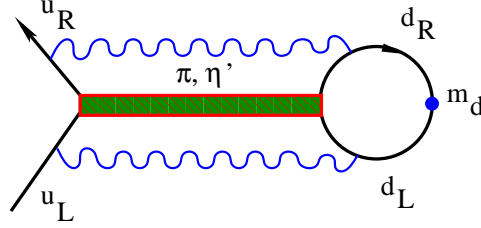
Fig. 10.5. Through physical meson exchange, a down quark mass can induce an effective mass for the up quark. The gluon exchanges can compensate for the pseudoscalar nature of the meson fields. Figure from Ref. [99].
