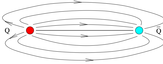
Fig. 1.1. A tube of gluonic flux connects quarks and anti-quarks. The strength of this string is 14 tons.
