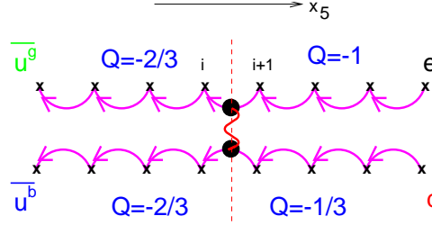
Fig. 13.4. Transferring charge between the doublets. Figure taken from [180].
