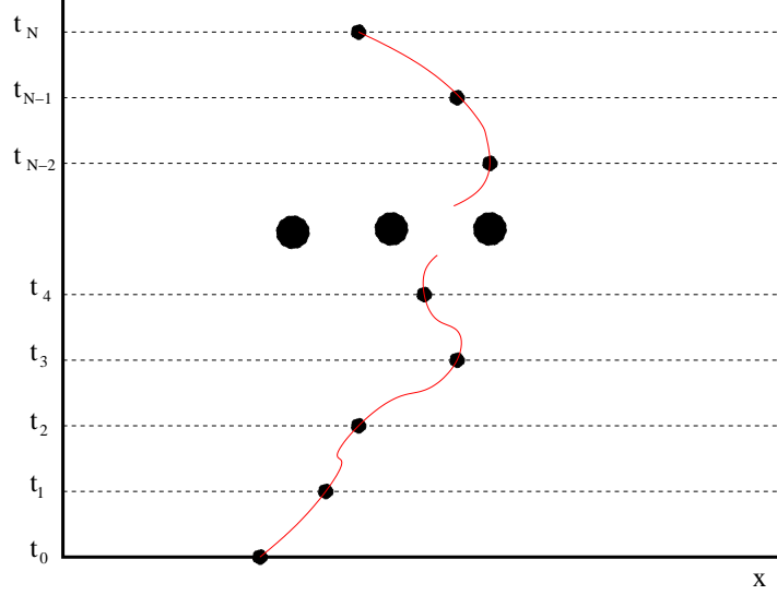
Fig. 2.1. Dividing time into a lattice of N slices of timestep a .
