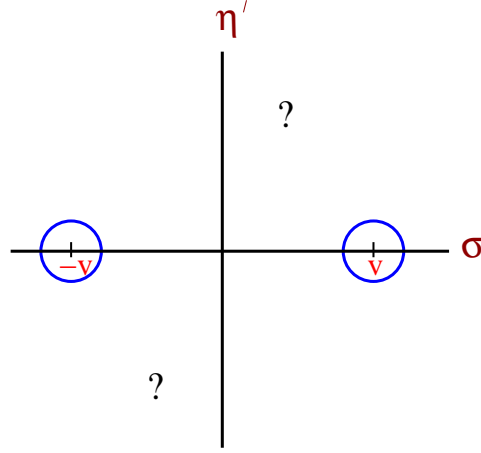
Fig. 9.1. We have two minima in the \sigma, \eta' plane located at \sigma = \pm v and \eta' = 0 . The circles represent that the fields will fluctuate in a small region about these minima. Can we find any other minima?
