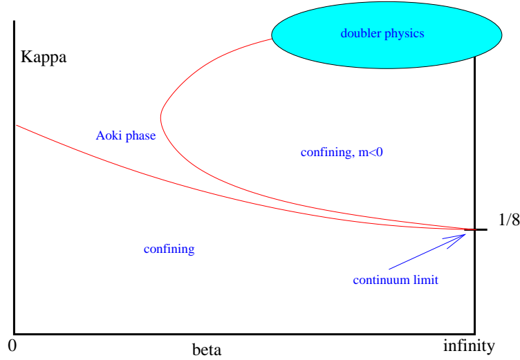
Fig. 11.5. The qualitative structure of the \beta, K plane including the possibility of an Aoki phase.
