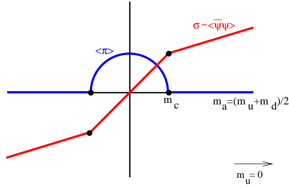
Fig. 10.8. With a constant up-down quark mass difference, the jump in the chiral condensate splits into two second order transitions. The order parameter distinguishing the intermediate phase is the expectation value of the neutral pion field. Figure taken from Ref. [106].
