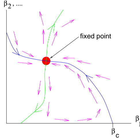
Fig. 6.2. A generic renormalization group flow. In general this occurs in an infinite dimensional space.
