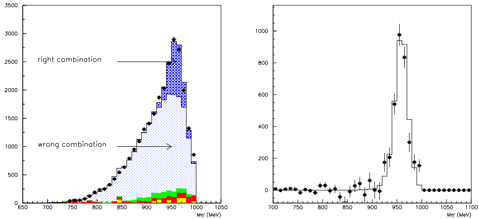
Fig. 2. \eta' \rightarrow \eta\pi^+\pi^- (\pi^0\pi^0) decays with \eta \rightarrow \pi^0\pi^0\pi^0 (\pi^+\pi^-\pi^0) . Left-side: distribution of the invariant mass of all possible photon combinations; right-side: invariant mass distribution after background subtraction.
