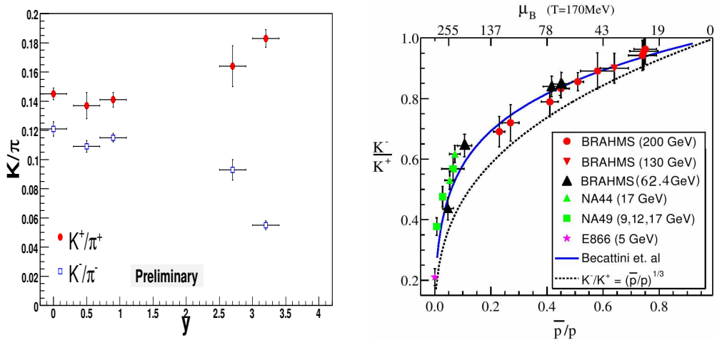
Fig. 5. Left: K^\pm/\pi^\pm ratios vs. rapidity; Right: Correlation between K^-/K^+ and \bar{p}/p ratios using data coming from a wide energy interval [2]. The solid curve is a statistical model calculation with a chemical freeze-out temperature fixed to 170 MeV but allowing the baryo-chemical potential to vary [6].
