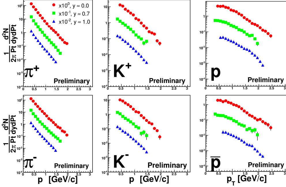
Fig. 1. Spectra for identified particles ( \pi^{+/-} , K^{+/-} , p^{+/-} ) at rapidities 0.0; 0.7 and 1.0. The distributions are scaled with a constant factor to be better viewed.
