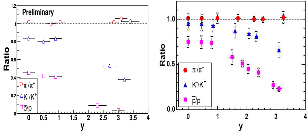
Fig. 3. \pi^-/\pi^+ , K^-/K^+ , \bar{p}/p ratios vs. rapidity in Au+Au collisions. Left: \sqrt{s_{NN}} = 62.4 \text{ GeV} ; Right: \sqrt{s_{NN}} = 200 \text{ GeV} [2].
