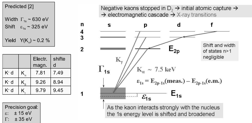
Fig. 2. Overview: X-ray transitions and strong interaction observables in kaonic deuterium.
