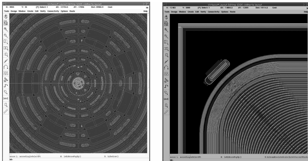
Fig. 4. Chip layout for SIDDHARTA, developed at PNSensor and MPE. SDD layout - readout side. Left: cell center. Right: cell edge.
