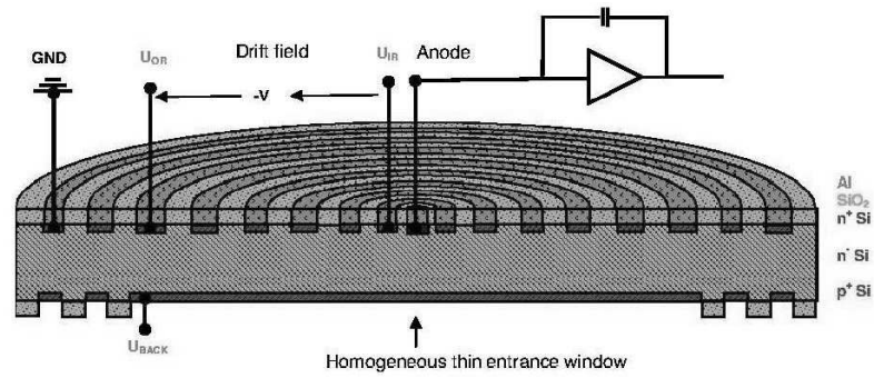
Fig. 3. Scheme of a Silicon Drift Detector with circular geometry.
