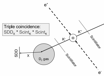
Fig. 1. Scheme of the triggered detection system for kaonic X-rays.
