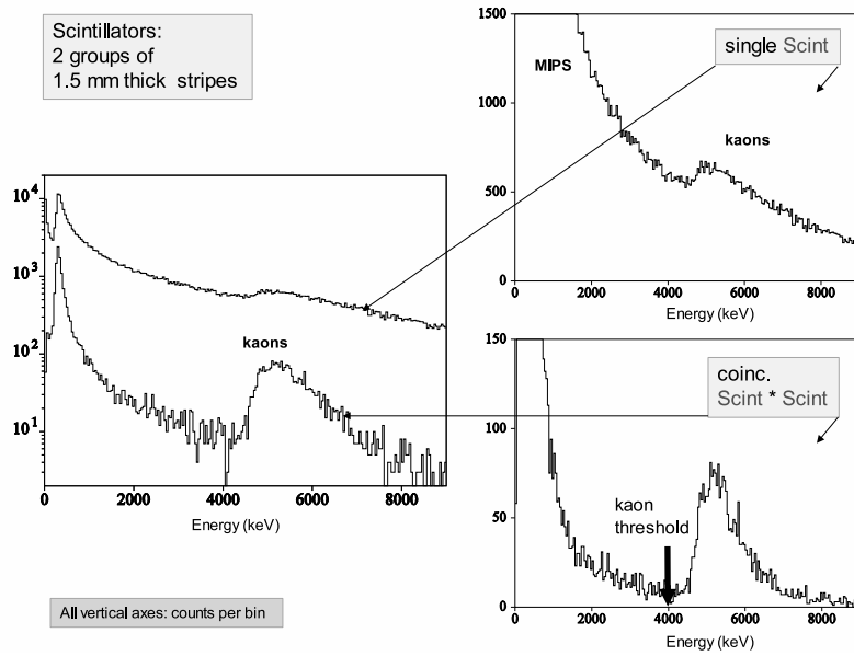
Fig. 7. Simulation of the energy signal of the trigger scintillators. Without usage of the fast back-to-back coincidence the kaon signal sits on a very high background ("single" spectrum).
