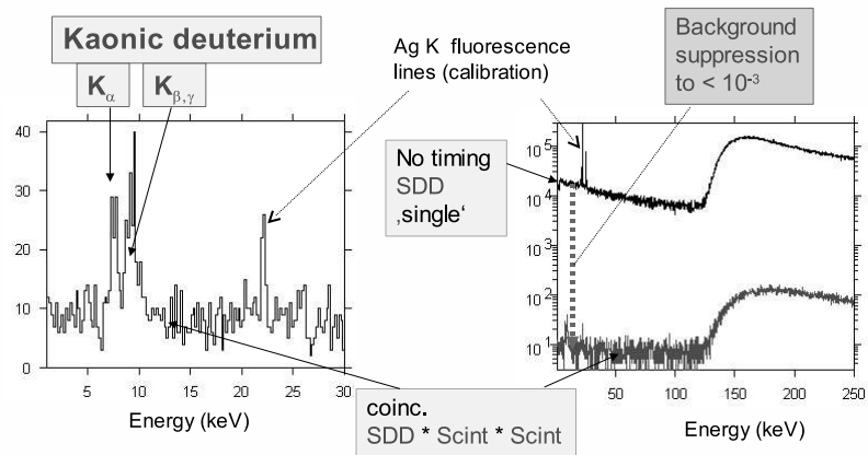
Fig. 8. Simulation of the energy signal of the SDDs. The rise of the spectrum above 120 keV corresponds to the energy MIPS deposit in 450 \mu\text{m} Si. The remaining background in the "coincidence" spectrum comes primarily from the decay of the charged kaons.
