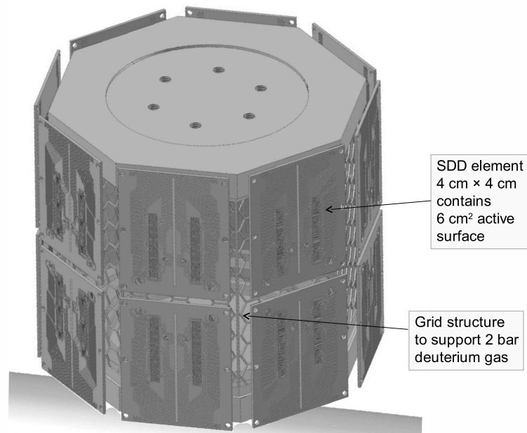
Fig. 5. Cell design. Trigger scintillators omitted
