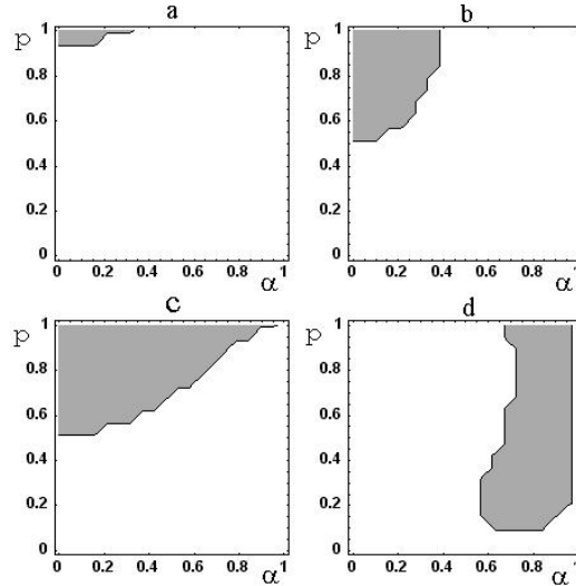
Fig. 1. Fidelity of the stabilization for depolarizing, \sigma_x , \sigma_y and \sigma_z channel. On the y axis is the parameter of the Pauli channel, on the x axis the parameter \alpha from the input state.
