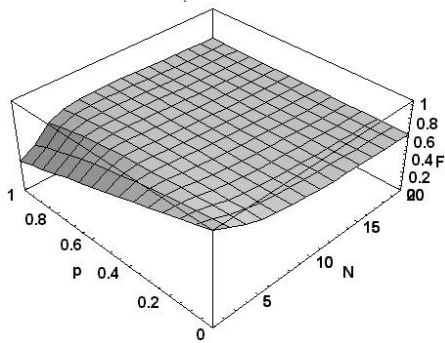
Fig. 2. Fidelity as the function of the probability of depolarasing Pauli channel and the number of qubits used. For N = 1 it is a simple acting of the Pauli channel on one qubit.
