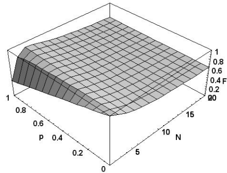
Fig. 3. The same as Fig. 2 but for \sigma_z channel.
