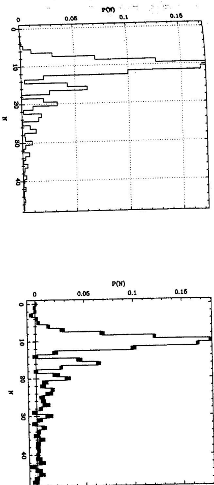
Fig. 2. We present an example for the reconstruction scheme based on Eqs (8) and (9). Fig. 2a shows the true photon-number distribution for a squeezed state with squeezing parameter s = 20 and displacement parameter \alpha = 3 , while Fig. 2b displays the distribution reconstructed from computer experiments using 260 quadrature phases with 100 simulated measurements for each phase. The errors indicated were obtained from 10 simulated runs.
